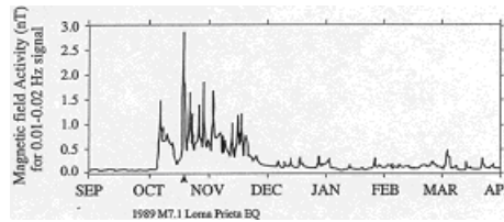
Magnetic data before & after the Loma Prieta earthquake in California, 1989.
